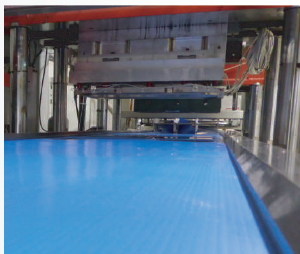
FIG.5 SIGNO sealing station.
